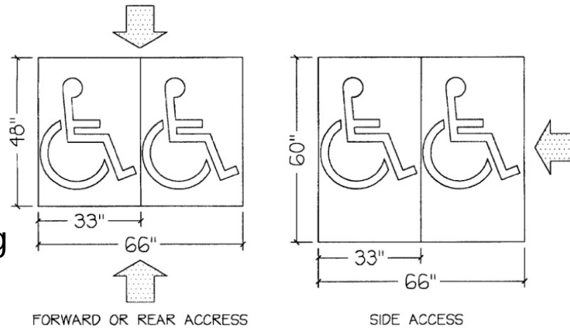
IBC TABLE 1108.2.2.1 ACCESSIBLE WHEELCHAIR SPACES
